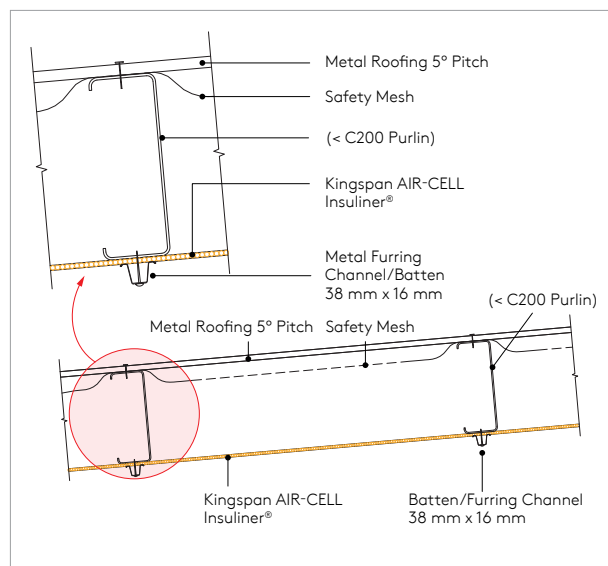
Figure 4. Side elevation of Kingspan AIR-CELL Insuliner® in a warehouse metal deck roof retrofit.
