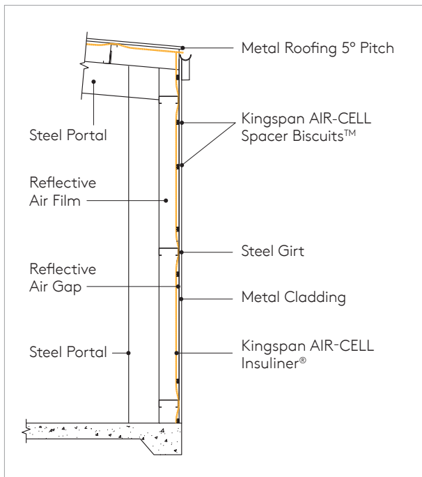
Figure 6. Side elevation of Kingspan AIR-CELL Insuliner® in a warehouse wall.
